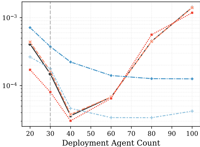
Robustness: Combined Low ( \sigma_u = 0.02, \sigma_z = 0.01 )
