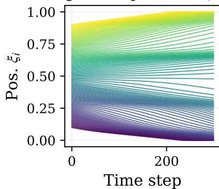
Agent Trajectories \xi_i(t)
