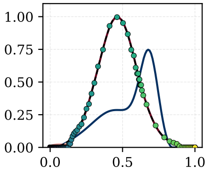
Velocity v_i(t)
