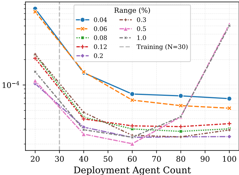
Sensor Range Sensitivity
