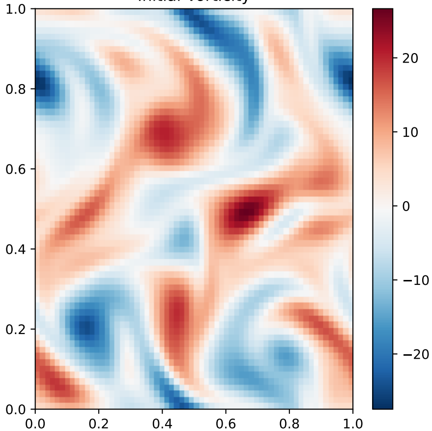
Initial Vorticity
