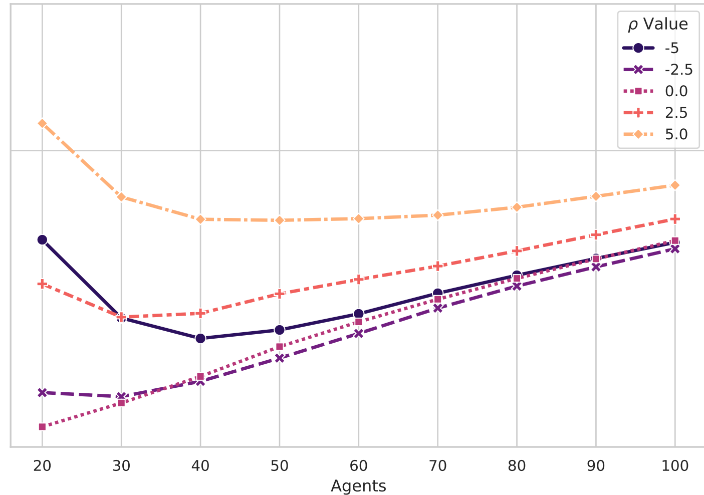
Sensitivity to Growth Rate ( \rho ) Fixed \nu = 0.005
