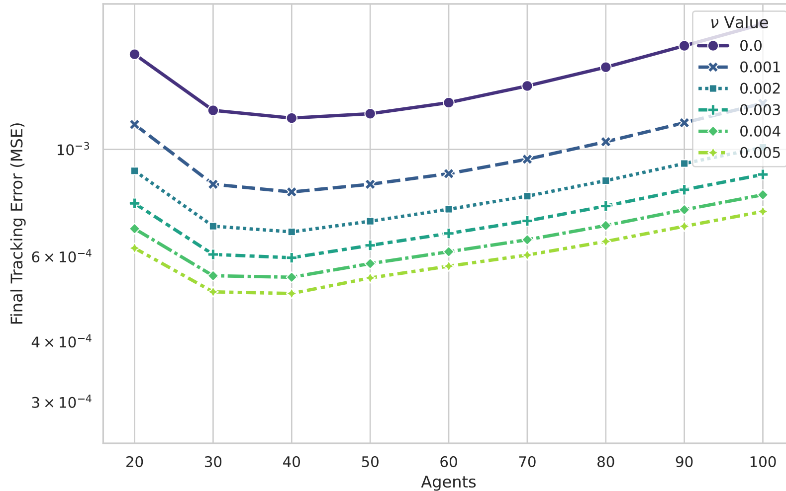
Sensitivity to Diffusion ( \nu ) Fixed \rho = 3.0
