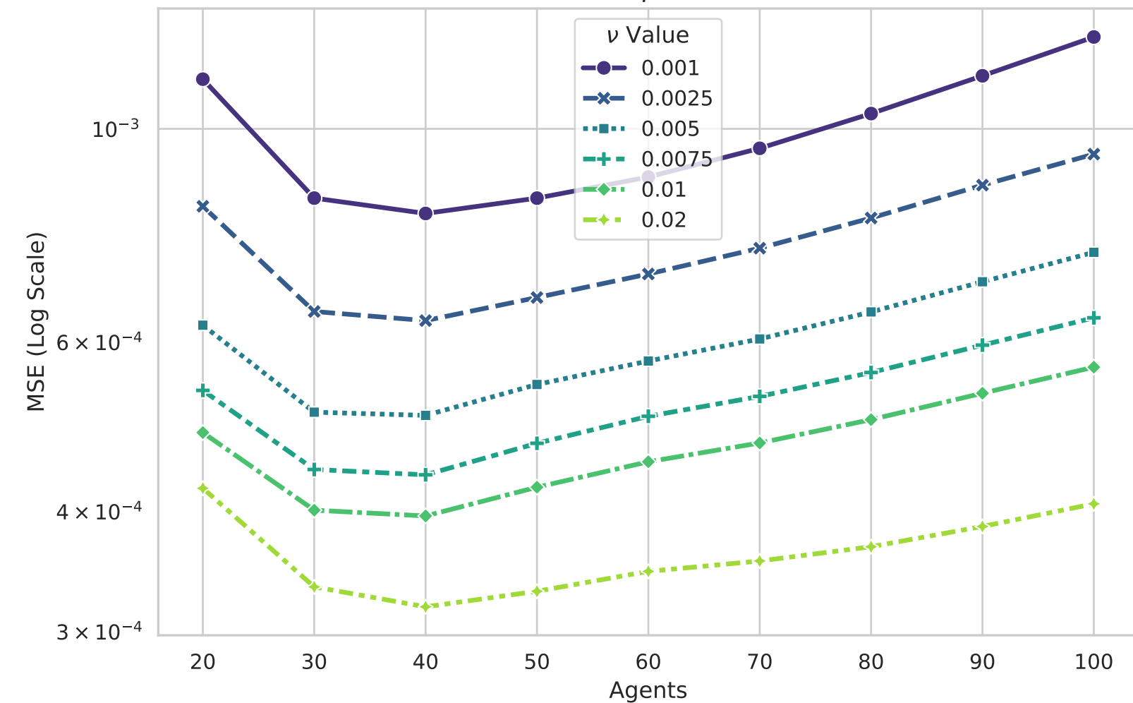
Ablation: Diffusion Coefficient ( \nu ) Fixed \rho = 3.0
