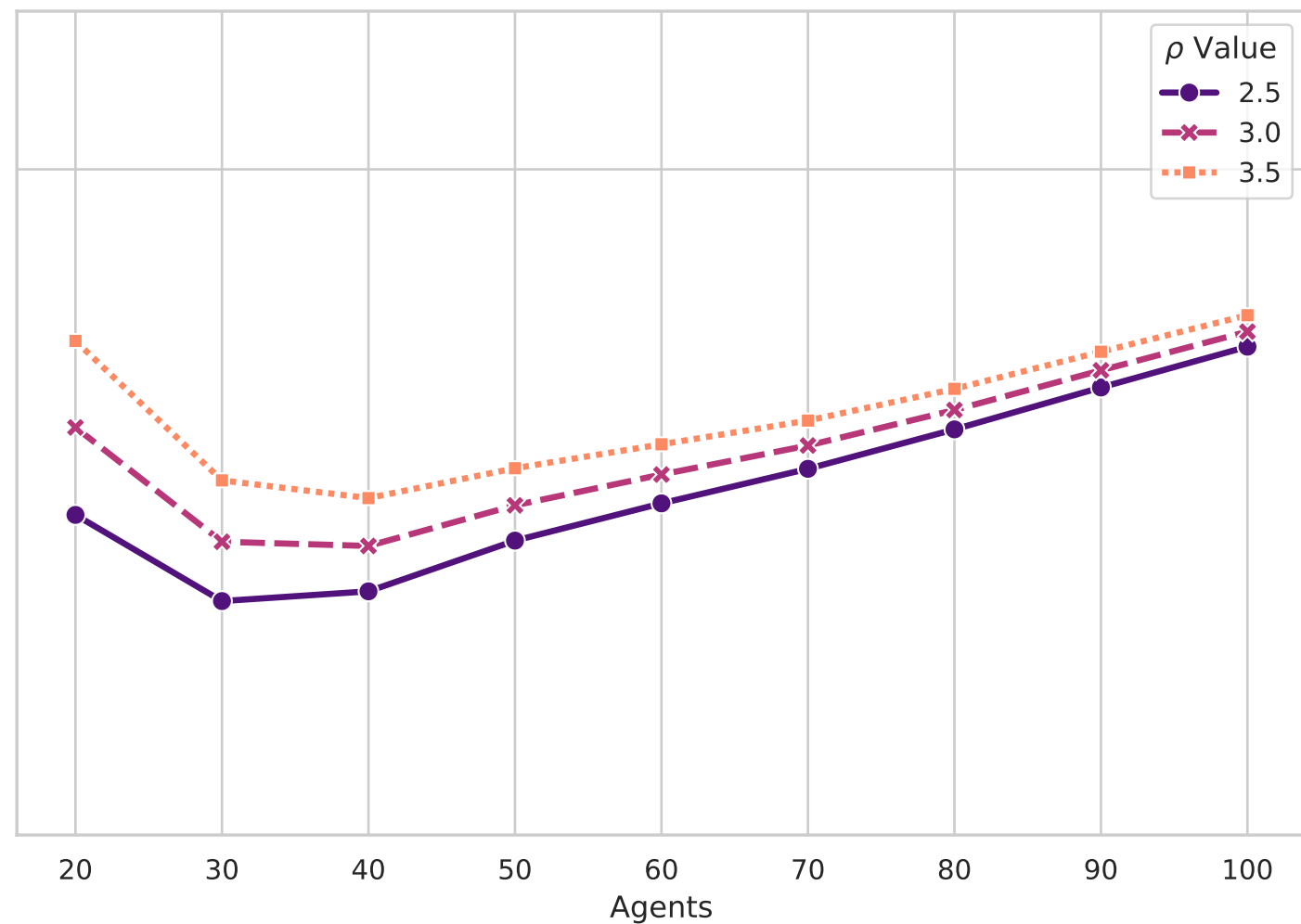
Ablation: Growth Rate ( \rho ) Fixed \nu = 0.005
