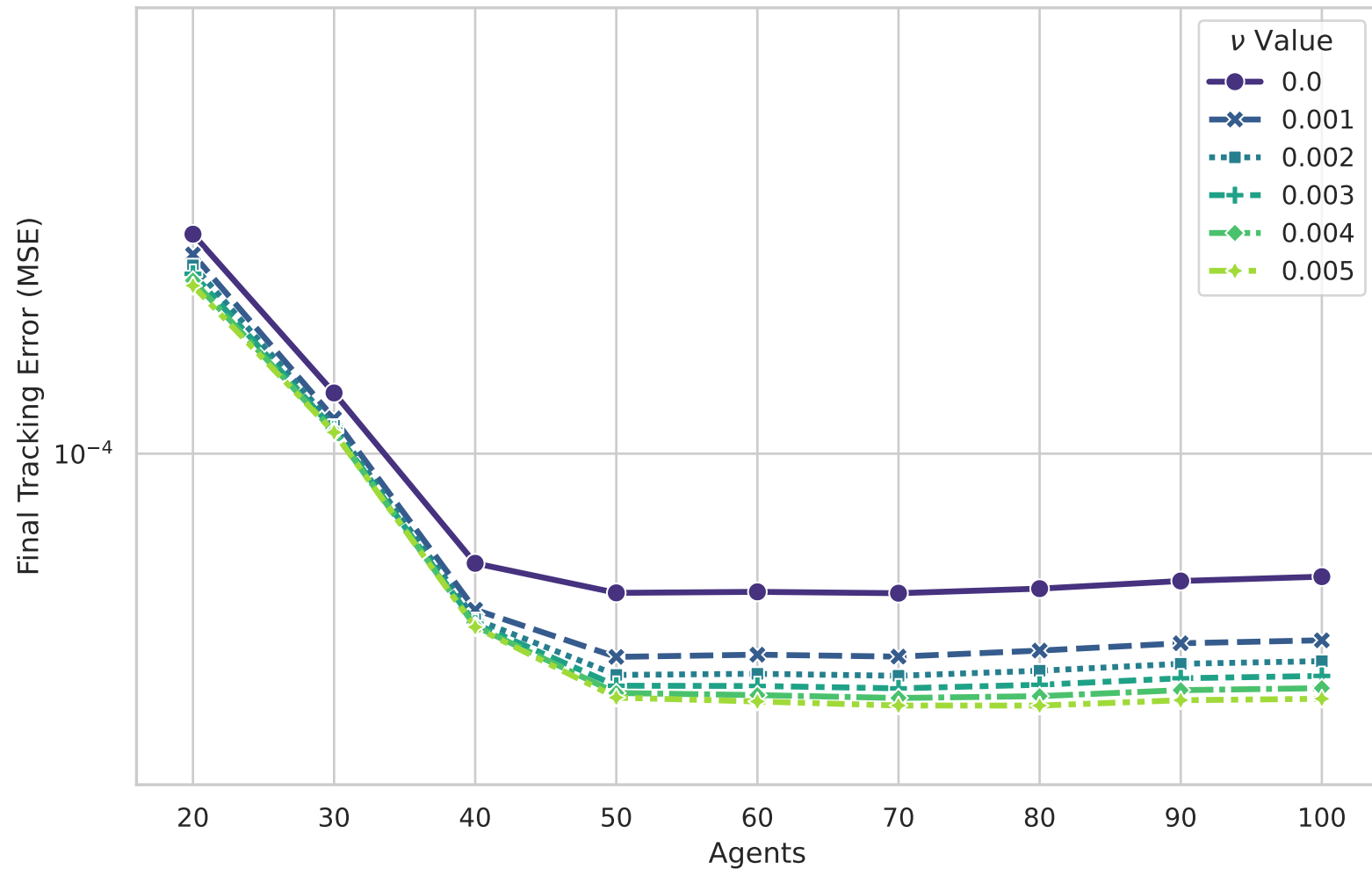
Sensitivity to Diffusion ( \nu ) Fixed \rho = 3.0
