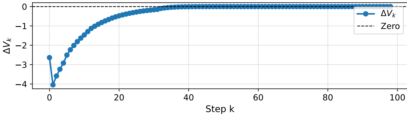
Lyapunov contract residual
