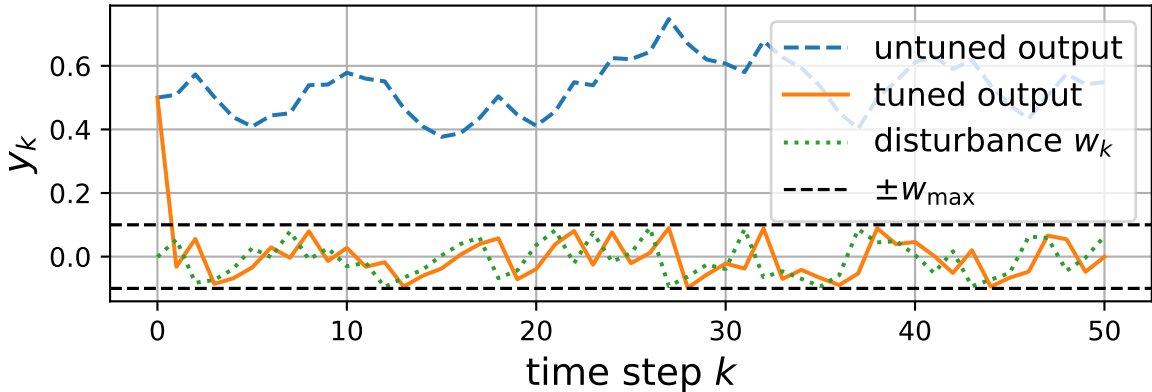
Closed-loop response with bounded disturbance
