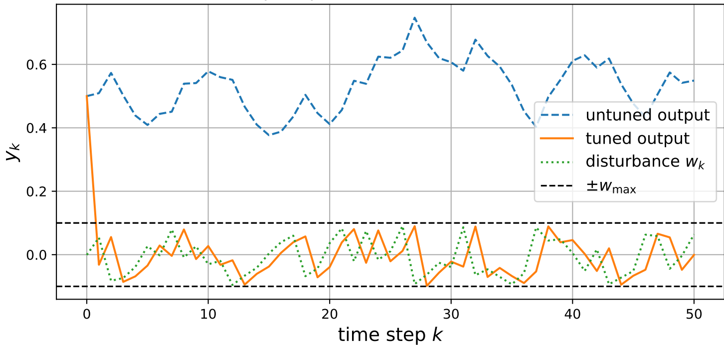
Closed-loop response with bounded disturbance
