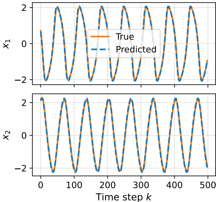
Learned Koopman trajectories
