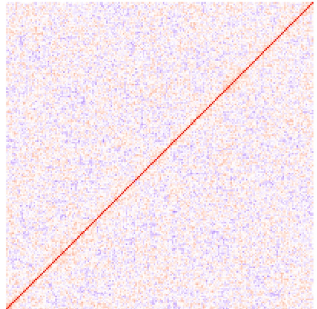
Simulated data, Parietal_Cell
