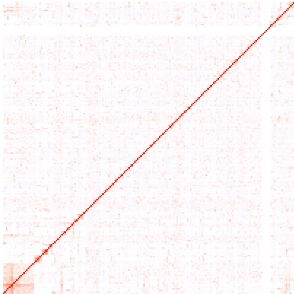
Real data, Parietal_Cell
