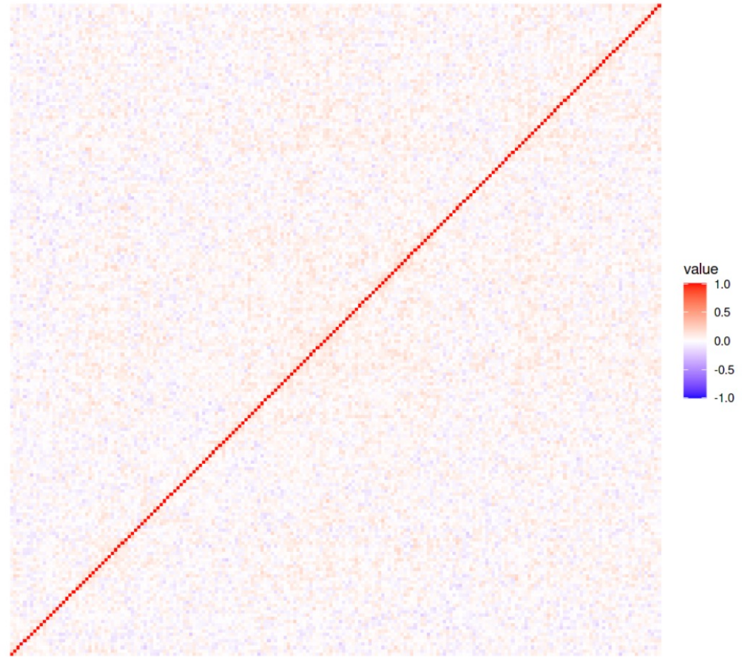
Simulated data, Esophageal_Epithelial_Cell
