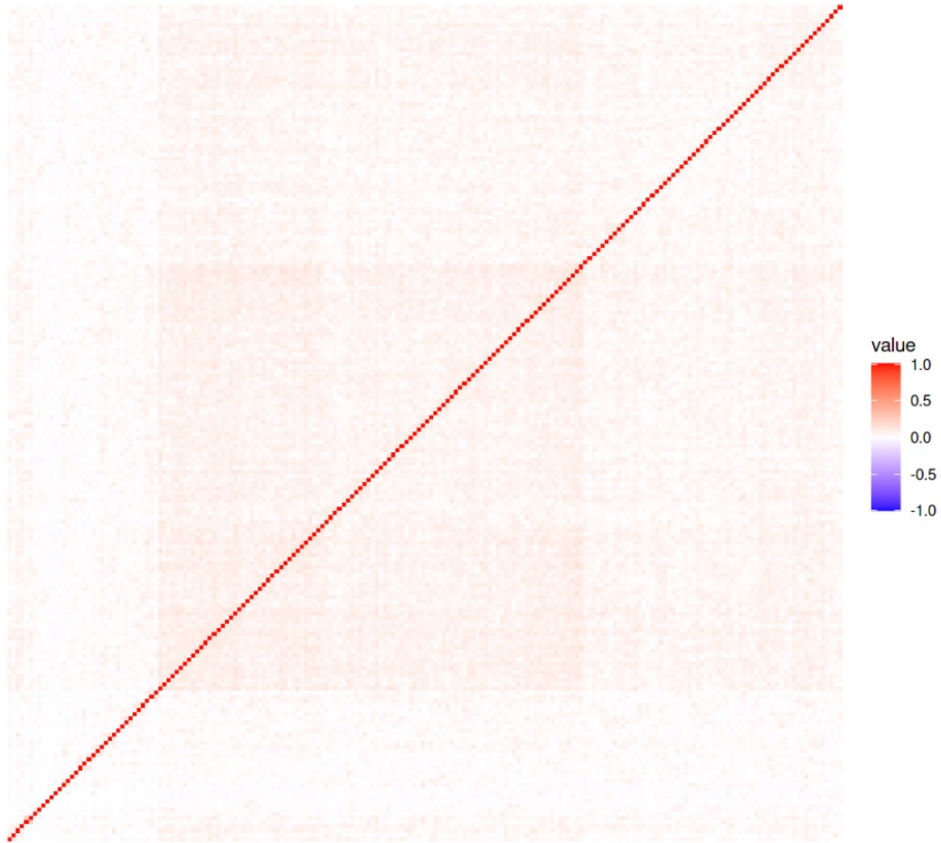
Real data, Esophageal_Epithelial_Cell
