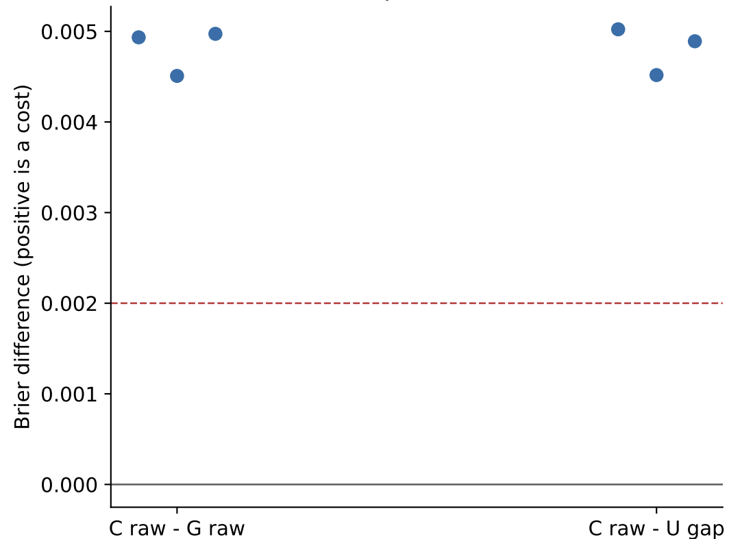
B Active prediction cost
