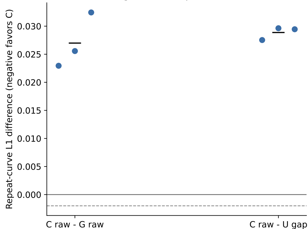
A Active generation: paired differences
