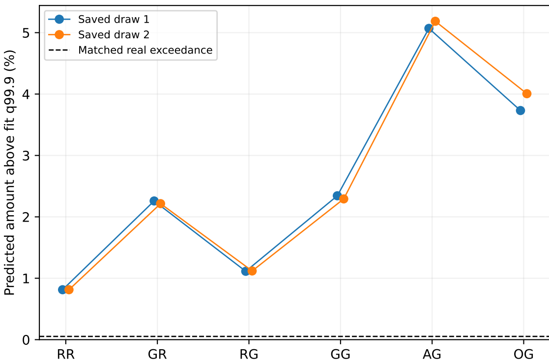
Frozen D: crossed histories and current gap/mark RR/GR/RG/GG: history/current; AG: generated past amount only; OG: generated other past fields Berka
