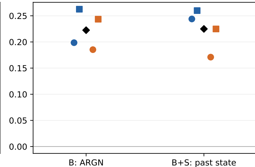
Customer length: log-W1
