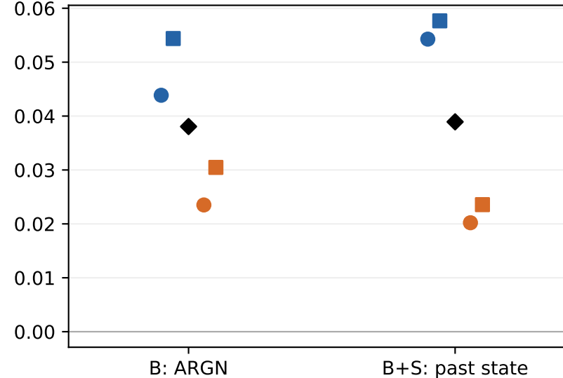
Normal amount: log-W1
