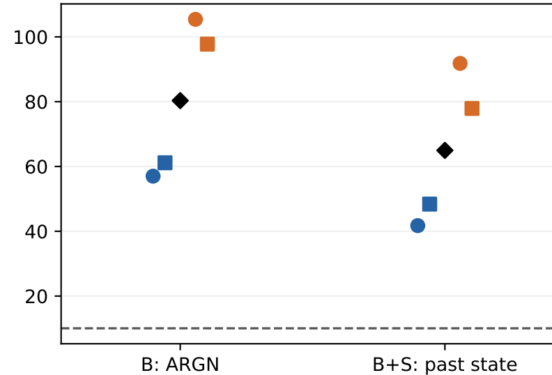
Normal amount: log-W1
