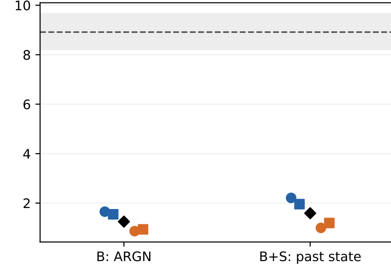
Customer length: log-W1
