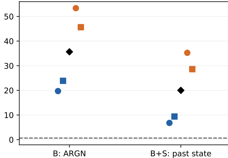
Fraud amount / past median: log-W1
