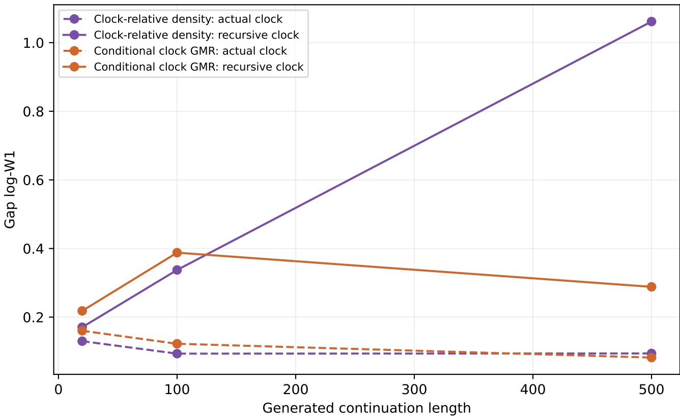
Same 105 customers, real prefix and oracle labels
