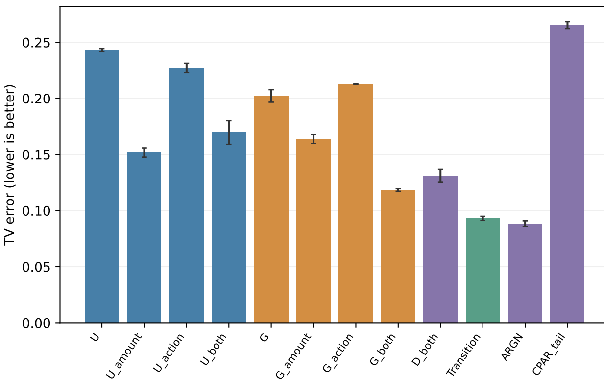
Sparkov: time-action relation
