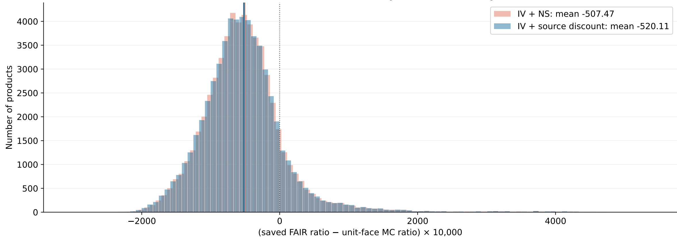
Discount-method control, 58,790 products; 40,000 paths
