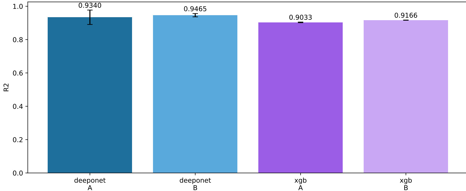
Stage-1 R2: rerun, 5 seeds mean \pm SD
