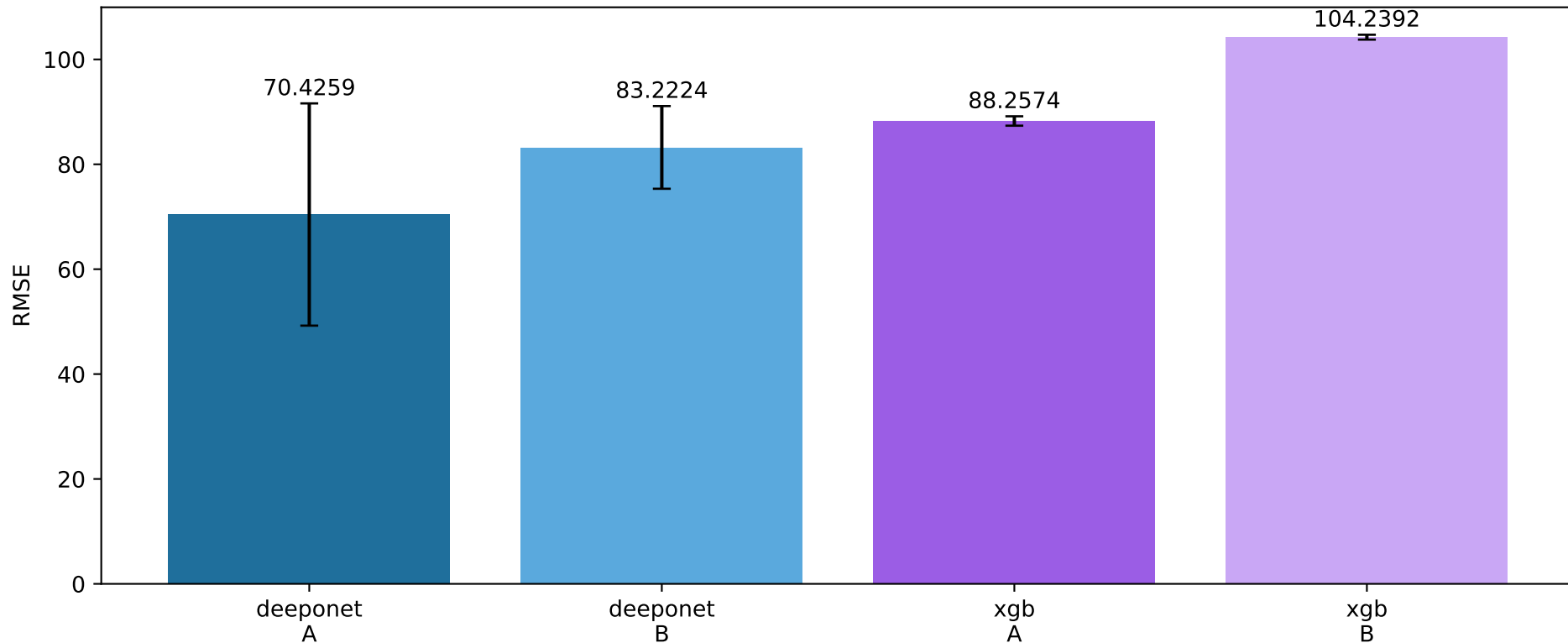
Stage-1 RMSE: rerun, 5 seeds mean \pm SD
