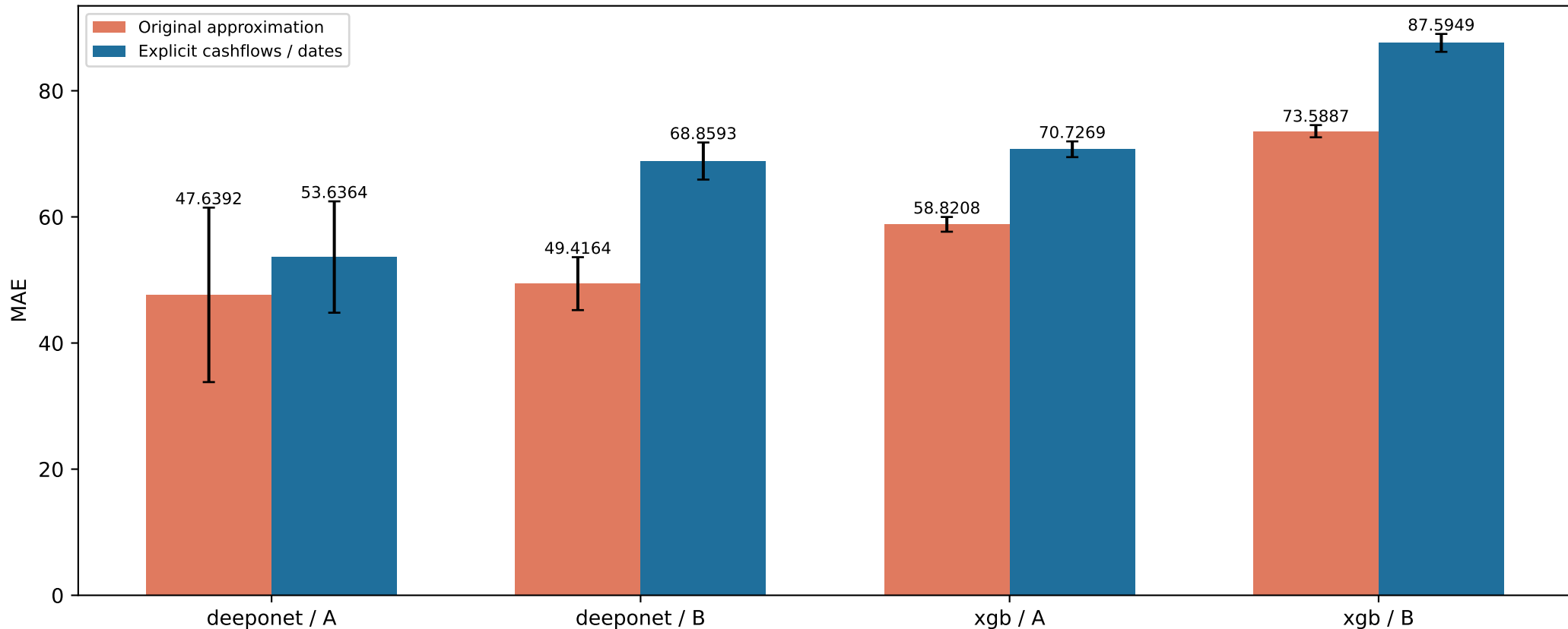
Stage-1 MAE: same sample / features, five seeds \pm SD
