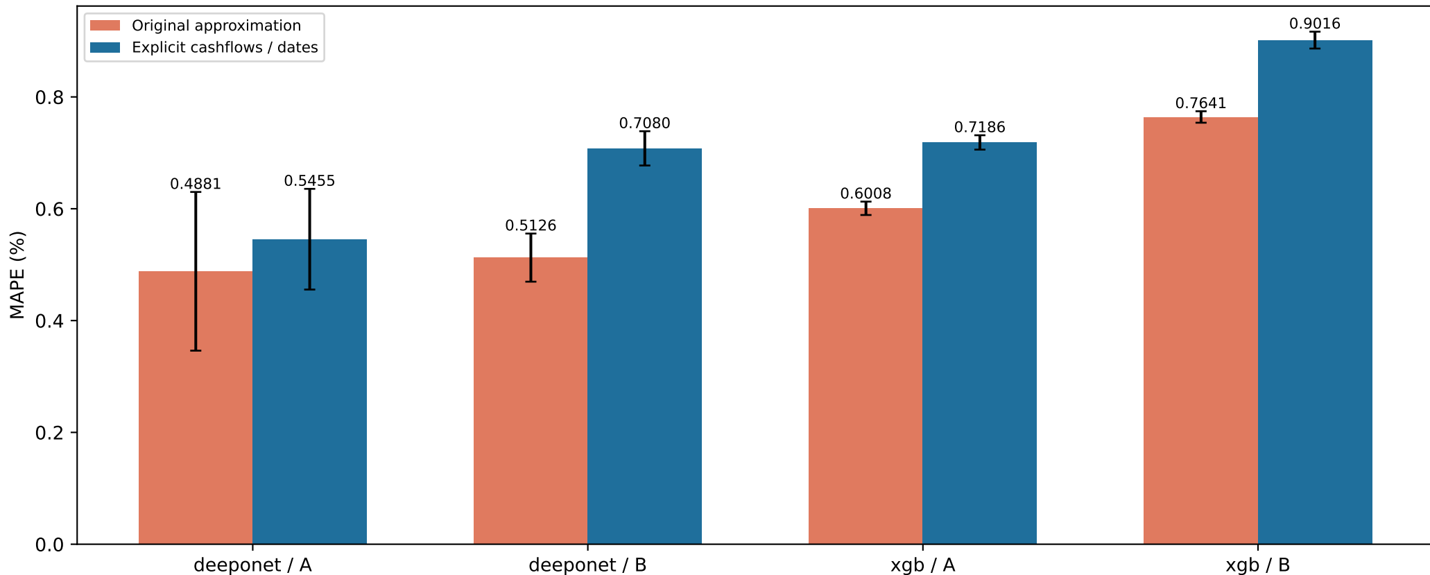
Stage-1 MAPE: same sample / features, five seeds \pm SD
