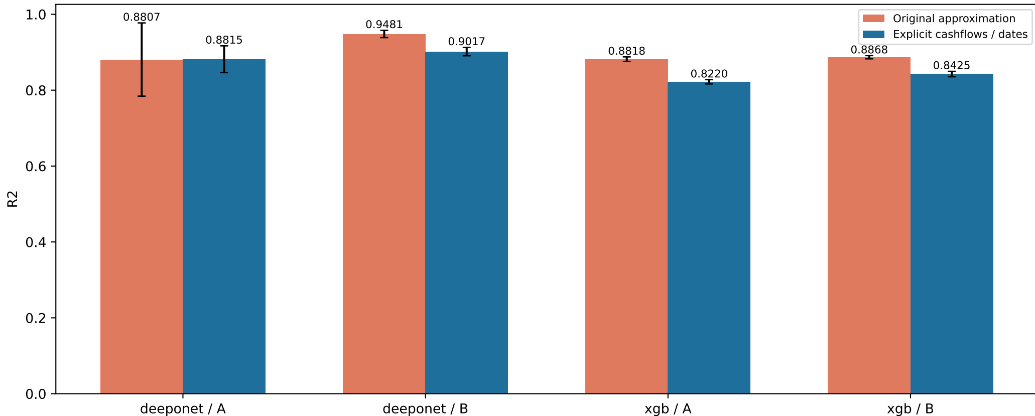
Stage-1 R2: same sample / features, five seeds \pm SD
