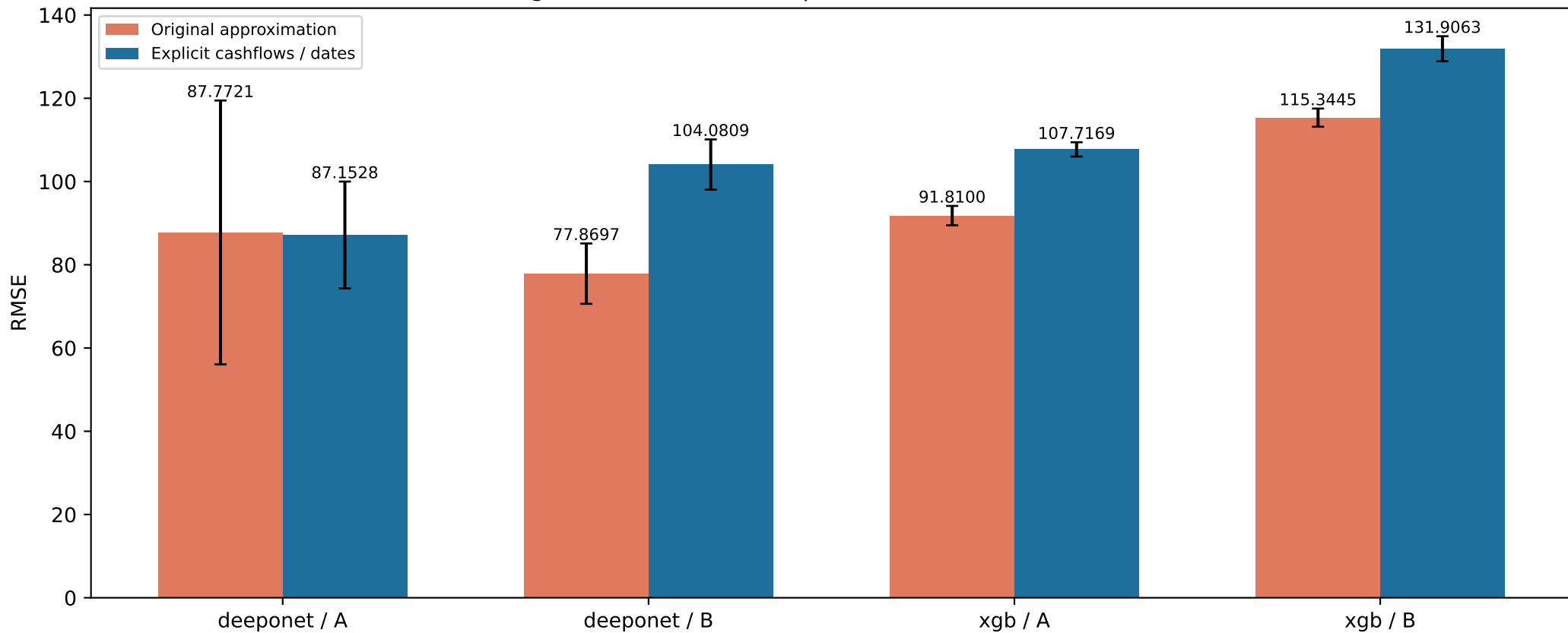
Stage-1 RMSE: same sample / features, five seeds \pm SD
