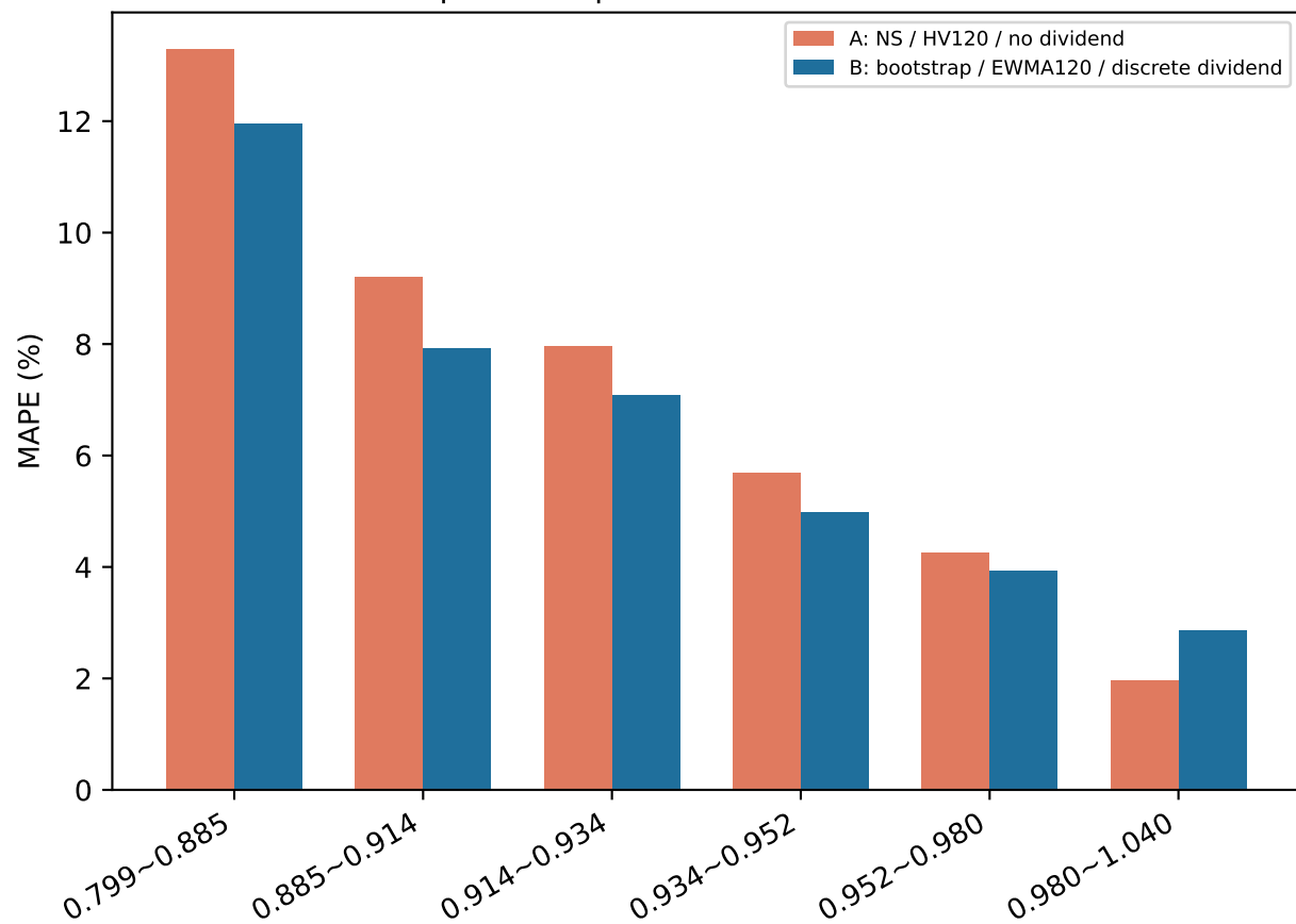
Mean |fair - MC| / fair: reconstructed n=200
