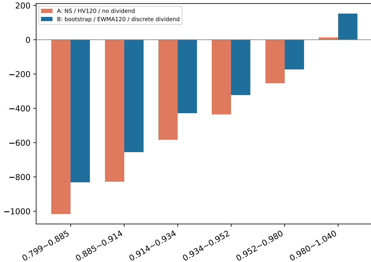
Mean fair - MC: reconstructed n=200
