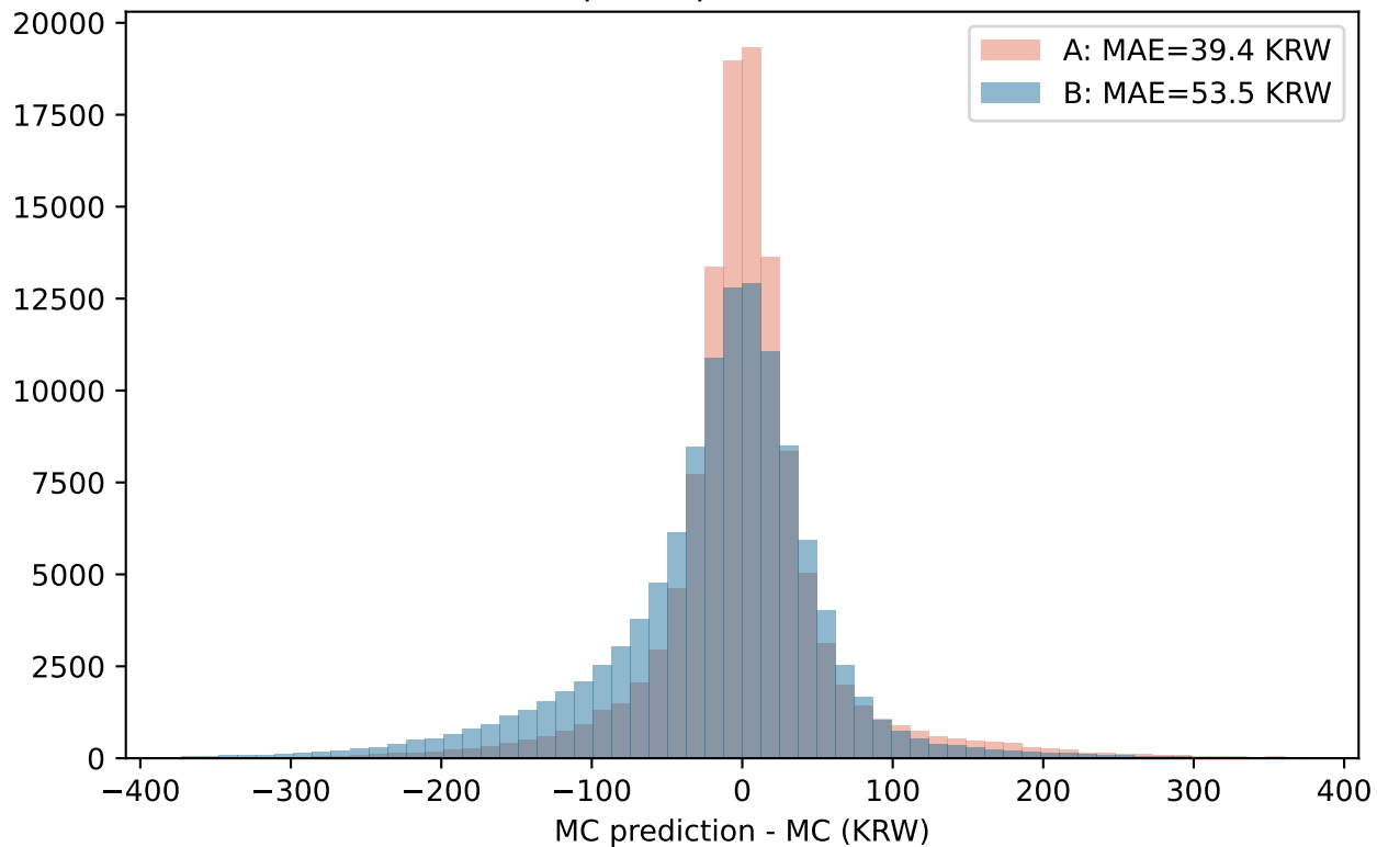
deeponet prediction error
