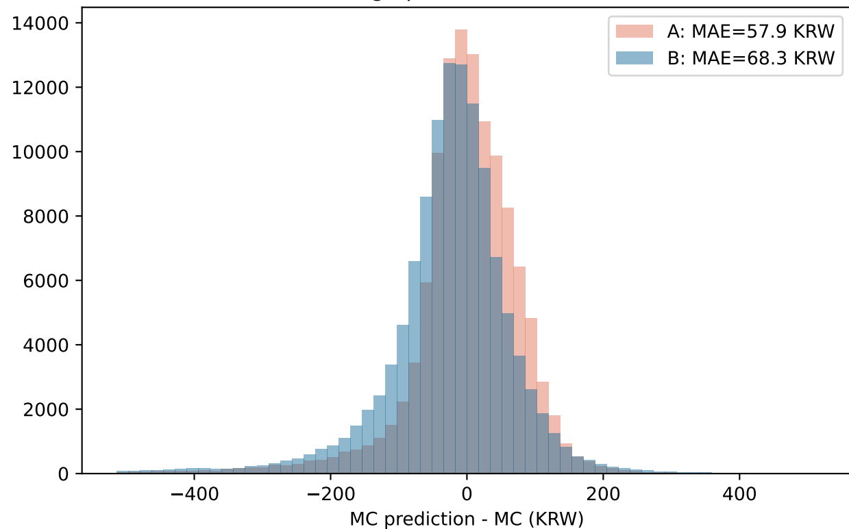
xgb prediction error
