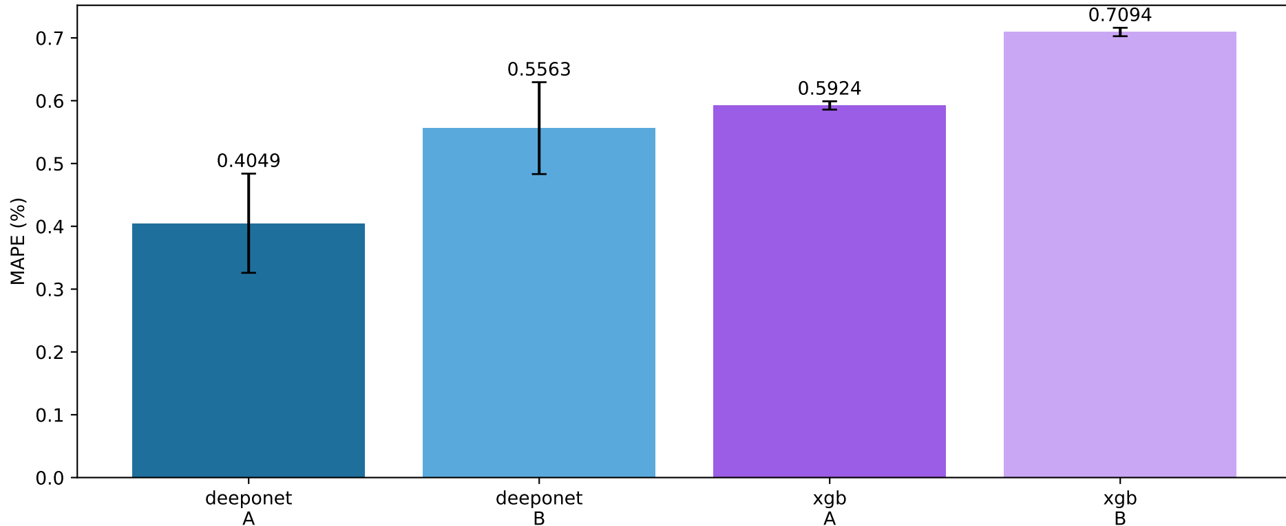
Stage-1 MAPE: rerun, 5 seeds mean \pm SD
