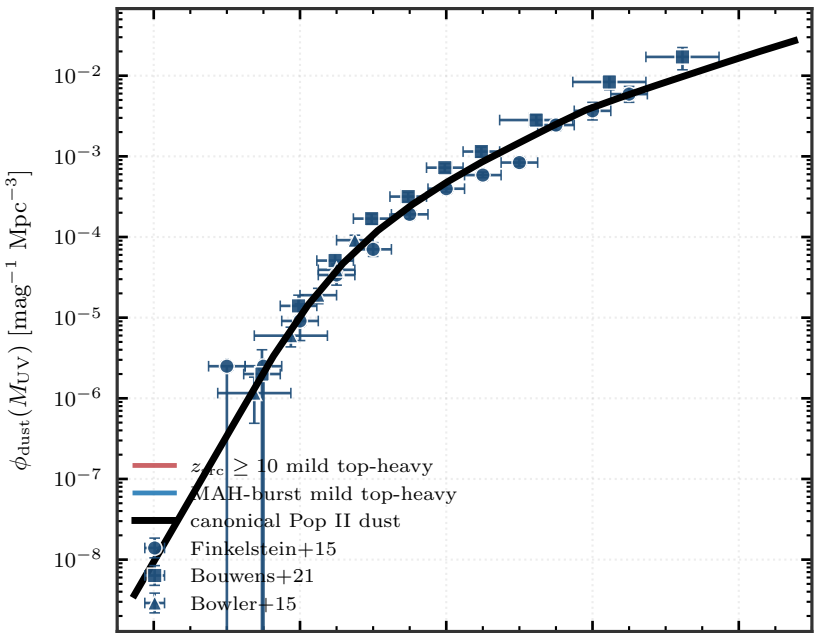
z = 6 dust-attenuated UVLF
