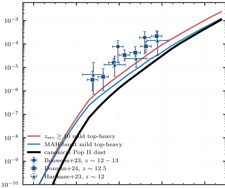
z = 12.5 dust-attenuated UVLF
