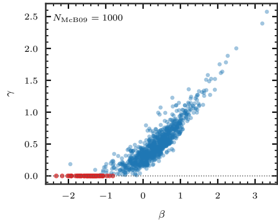
sampled McB09 parameters
