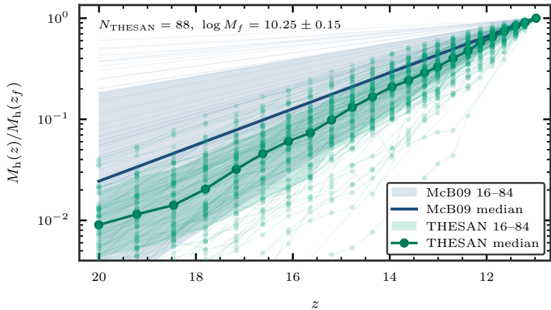
MAH shape at z_f = 10.98
