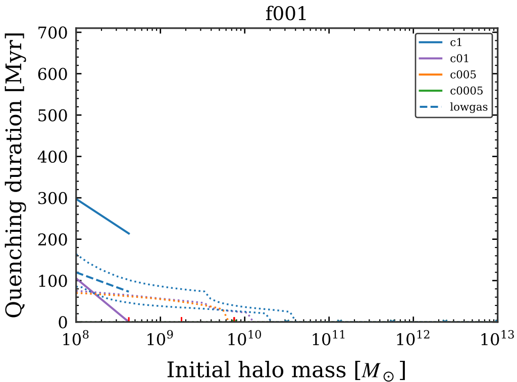
Fig. 8: full_approx; total gas accretion independent of covering fraction
