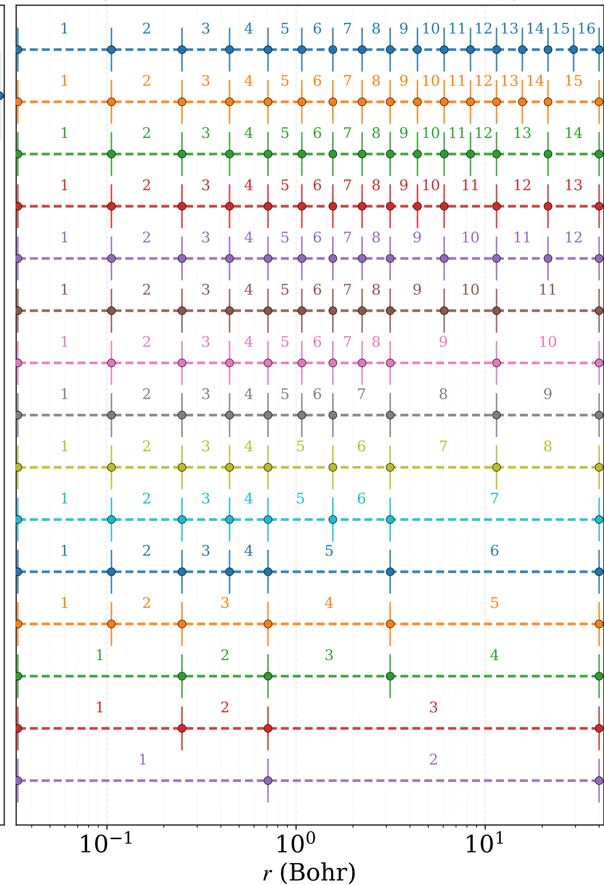
Finite-element sweep (coarsen interior nodes; same R_{\max} )
