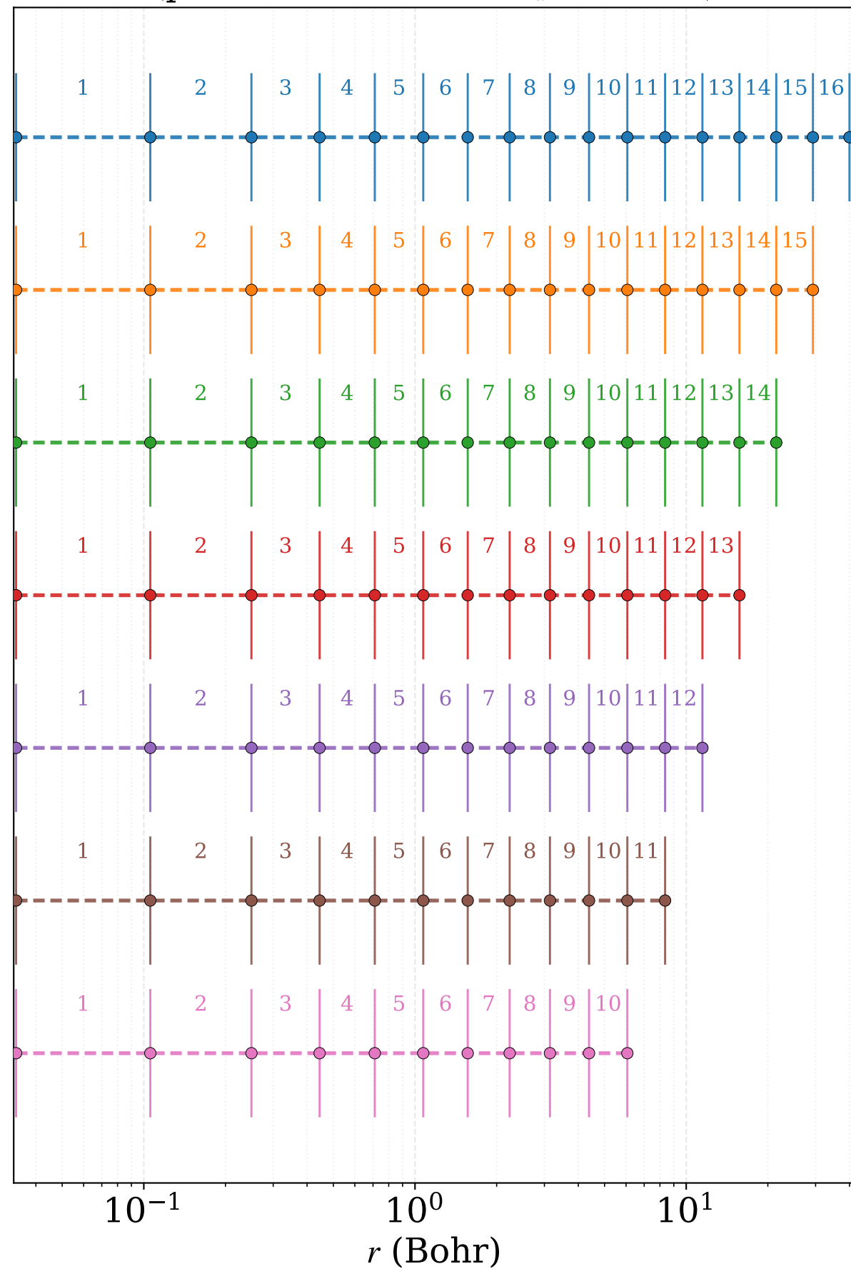
Domain-radius sweep (prefix boundaries; R_{\max} > 5 Bohr)
