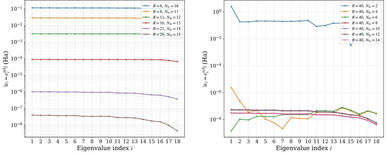
Figure 3: LDA-SVWN all-electron convergence for Z = 92 against FeAtom reference occupied eigenvalues at R_{max} = 40 Bohr and N_{fe} = 16 : absolute eigenvalue error versus R_{max} (left) and versus N_{fe} (right).
