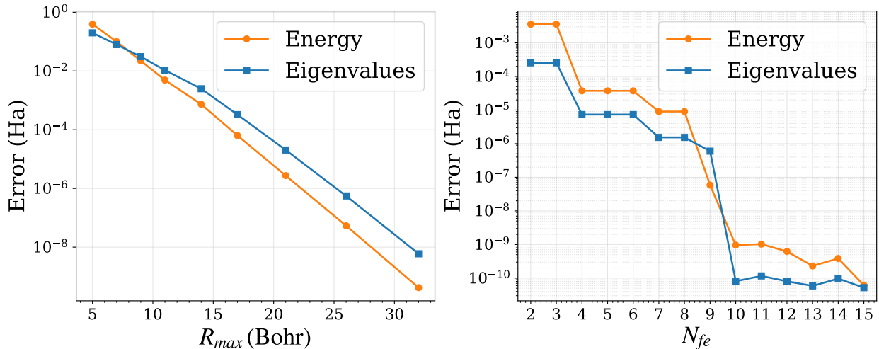
Figure 1: Convergence of the total energy and occupied valence eigenvalues with respect to domain size R_{max} (left) and number of finite elements N_{fe} (right) in pseudopotential Kohn–Sham DFT calculations, using the PBE exchange–correlation functional, for atomic numbers Z = 1\text{--}57 and Z = 72\text{--}83 . The energy error is defined as the maximum absolute total-energy difference over all atoms in the set, while the eigenvalue error is defined as the maximum, over those atoms, of the per-atom mean absolute difference in the occupied valence eigenvalues. Reference values are computed using domain size R_{max} = 40 Bohr and N_{fe} = 16 finite elements.
