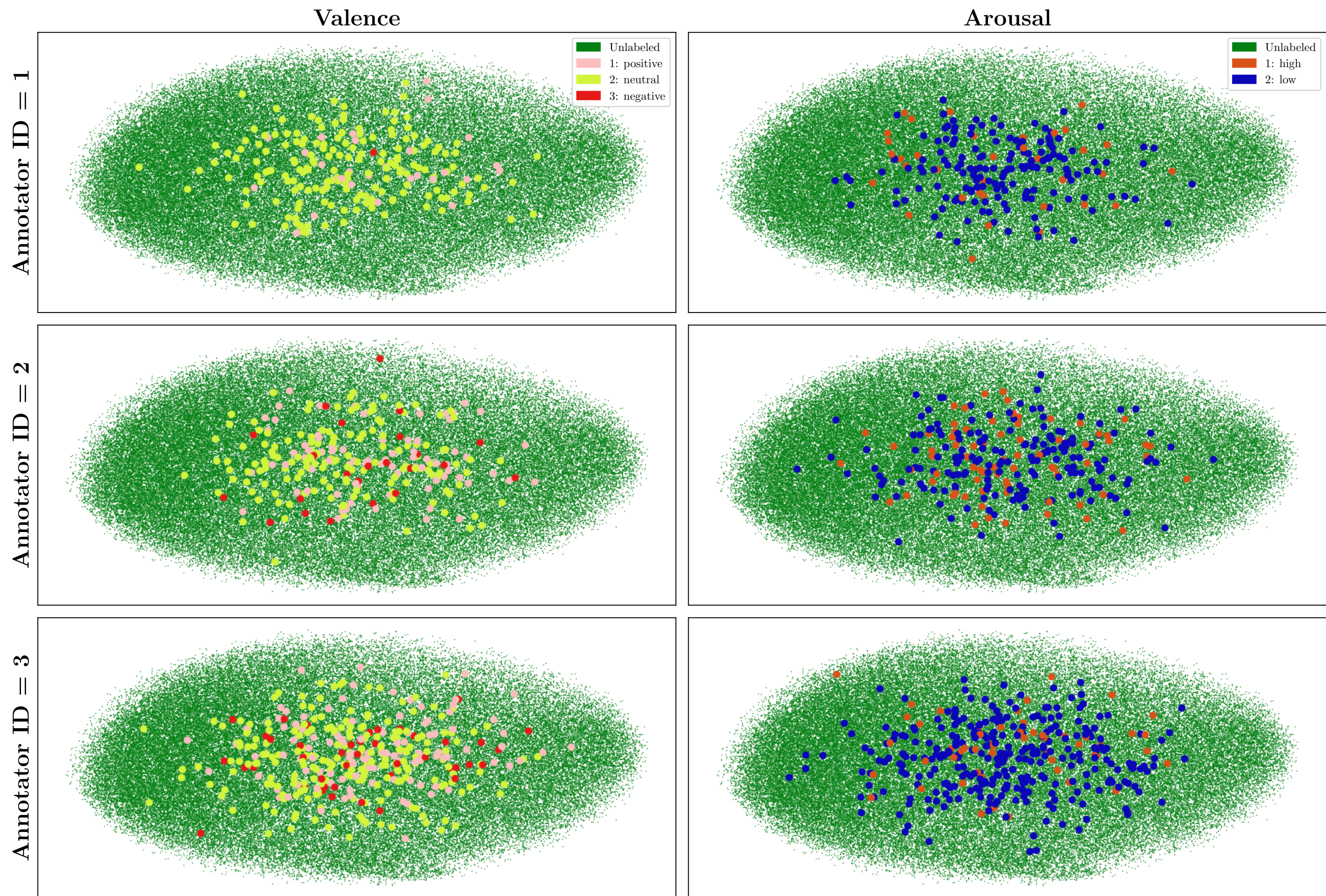
SER non-expert annotator label distributions by annotator ID, FAFT sample selection method (PCA visualization)
