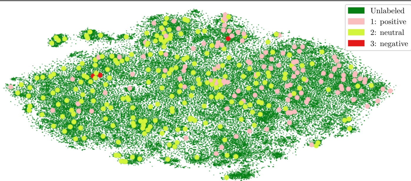
Valence
