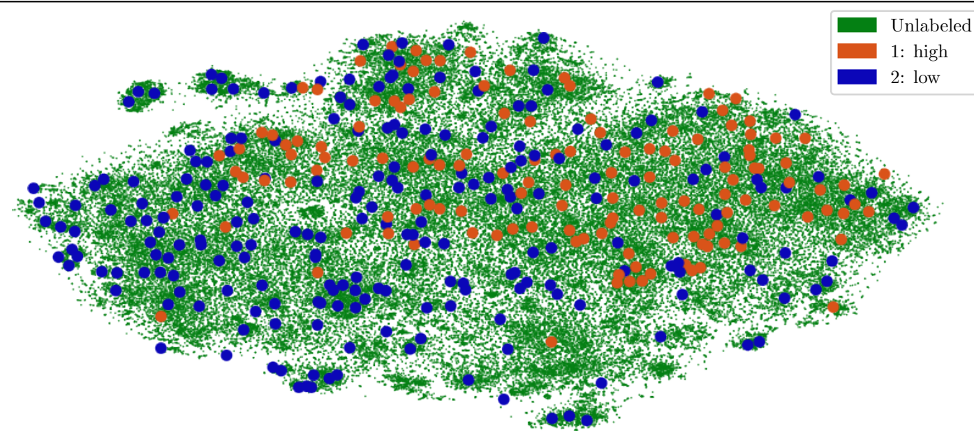
Arousal
