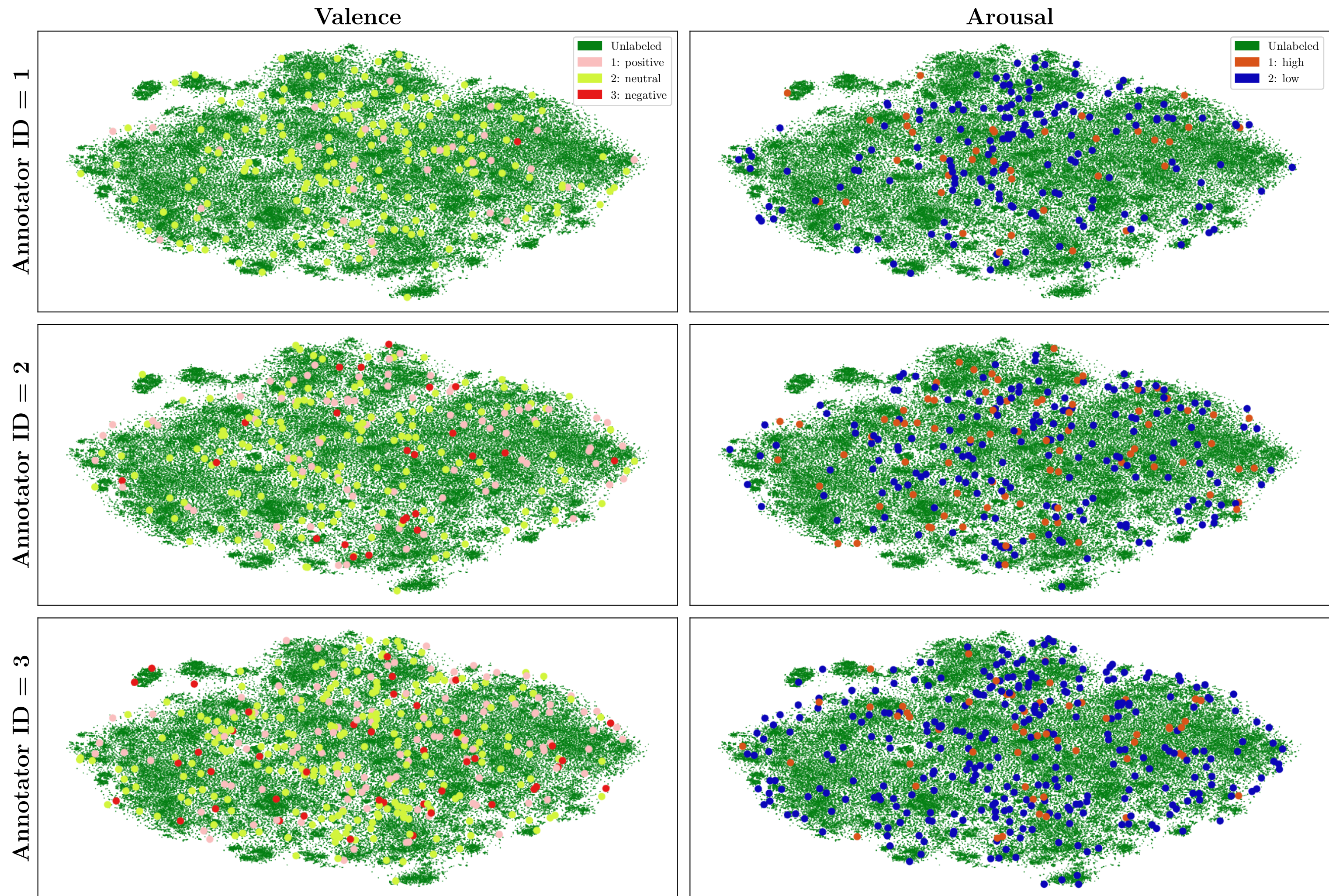
SER non-expert annotator label distributions by annotator ID, FAFT sample selection method (t-SNE visualization)
