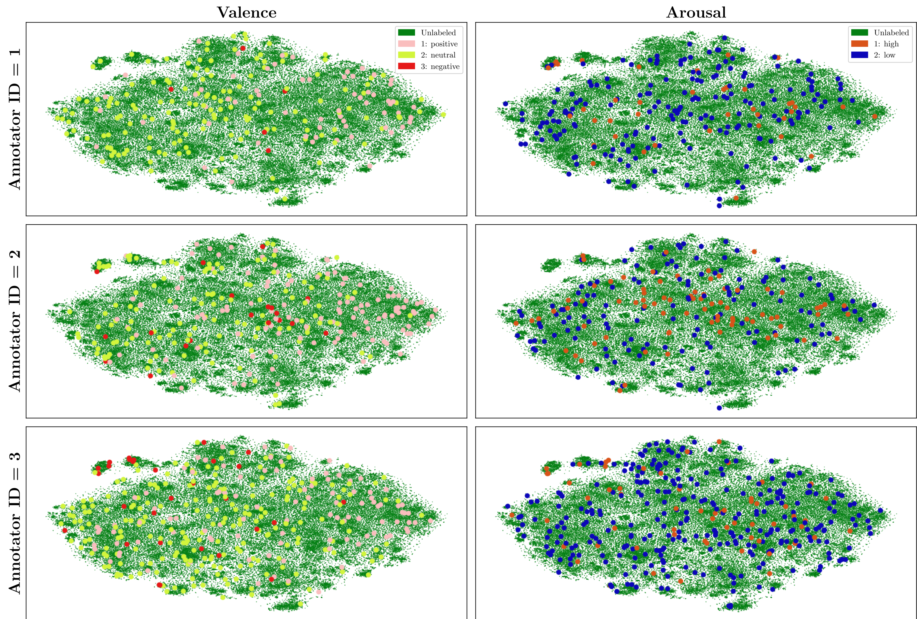
SER non-expert annotator label distributions by annotator ID, RND sample selection method (t-SNE visualization)
