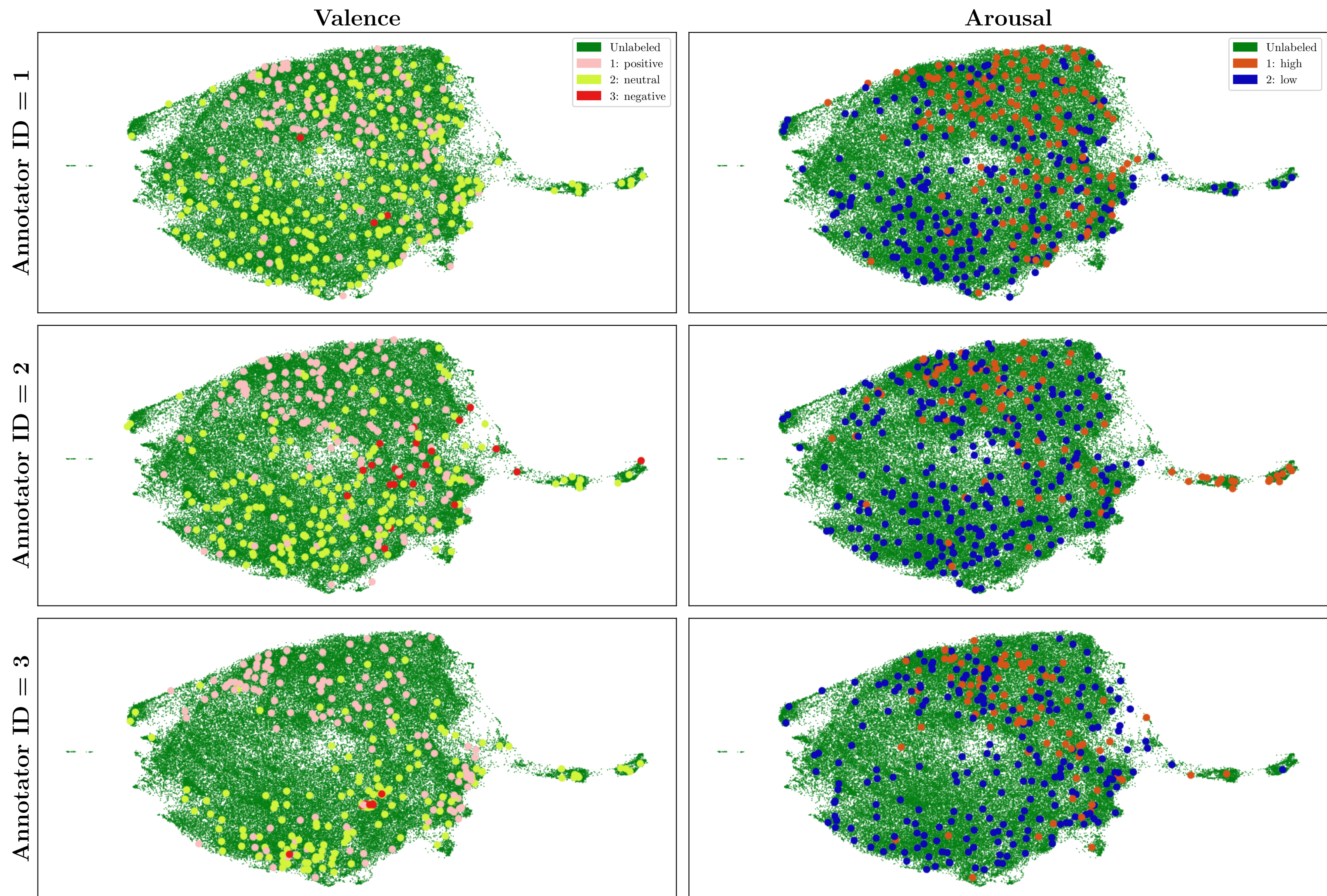
SER expert annotator label distributions by annotator ID, 2DV sample selection method (UMAP visualization)
