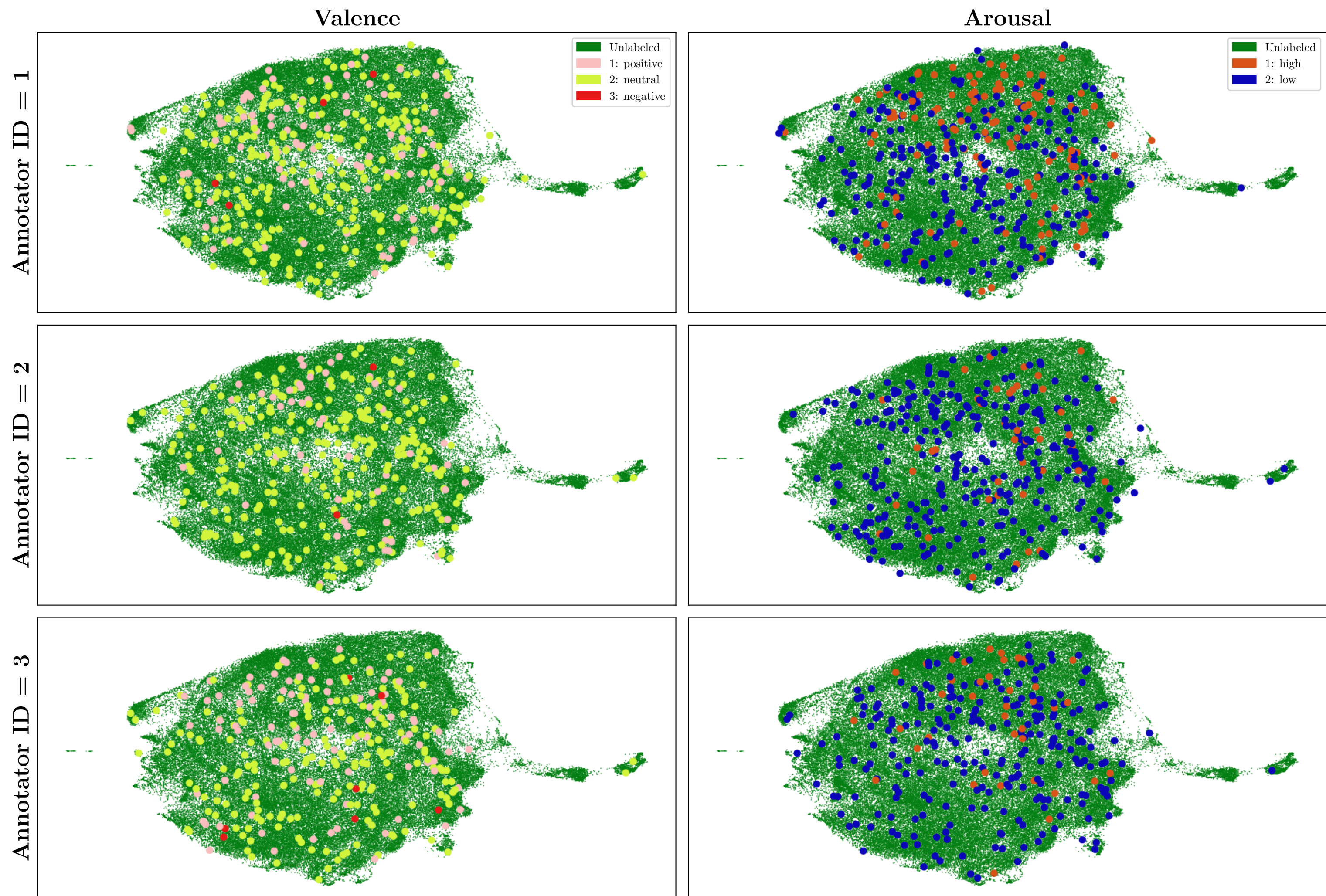
SER expert annotator label distributions by annotator ID, FAFT sample selection method (UMAP visualization)
