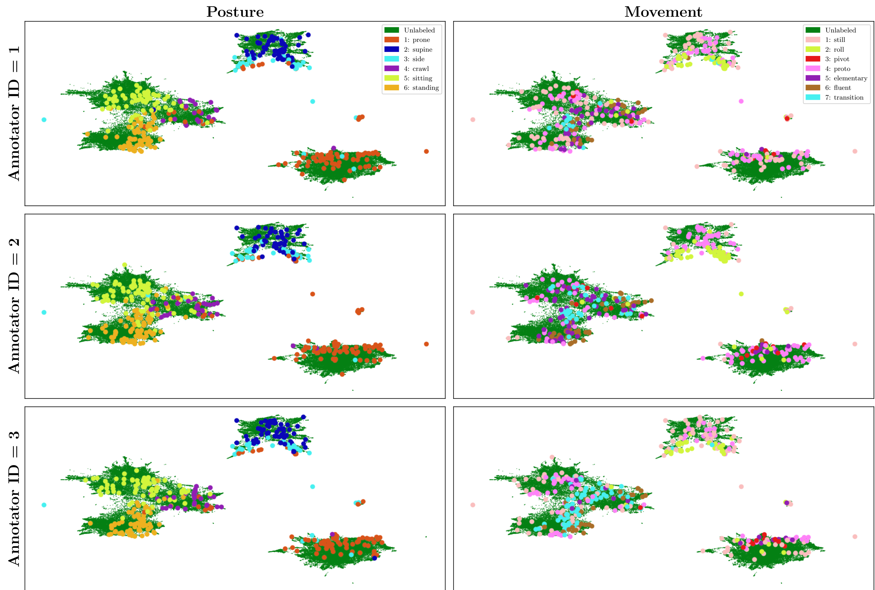
IMA non-expert annotator label distributions by annotator ID, FAFT sample selection method (UMAP visualization)
