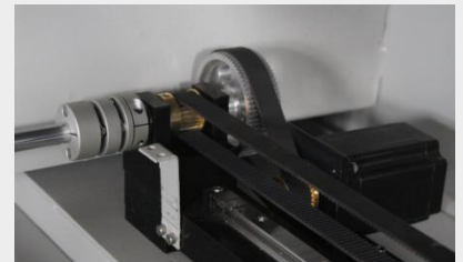
Guide rails and Fulong belt transmission
