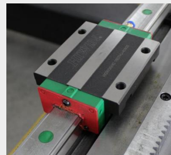
Taiwan-linear-guide-rail
