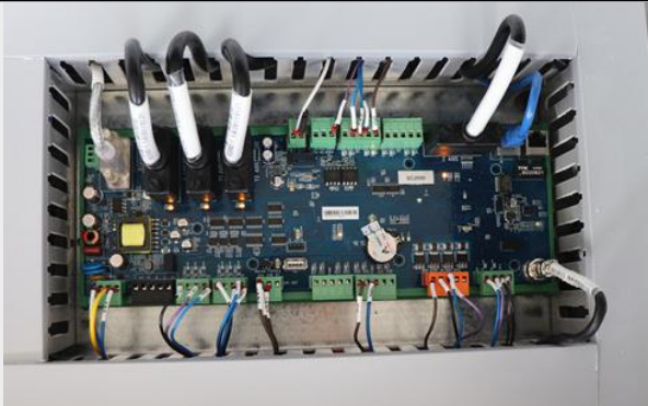
Au3tech Control board
