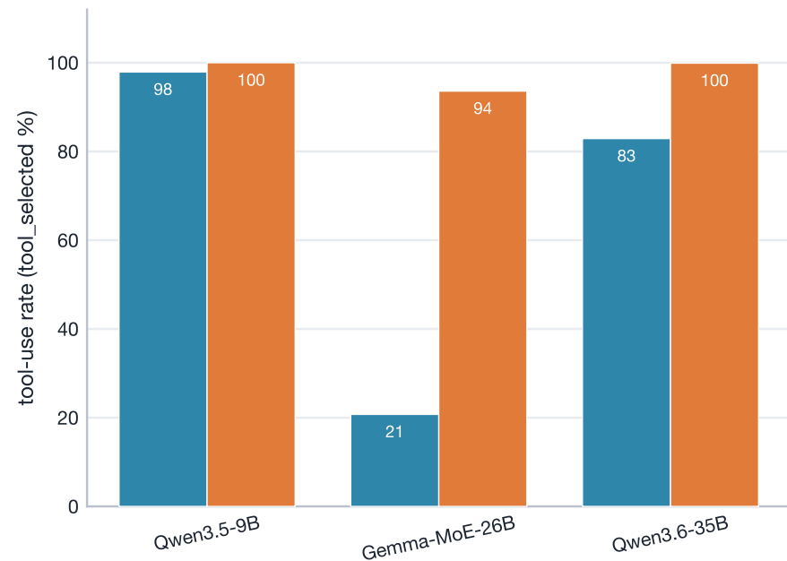
validate_plan — tool-use rate
