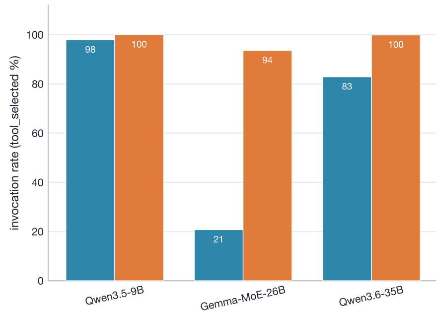
validate_plan — invocation rate
