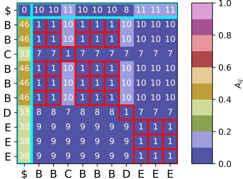
attention matrix
