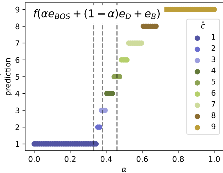
feedforward prediction
