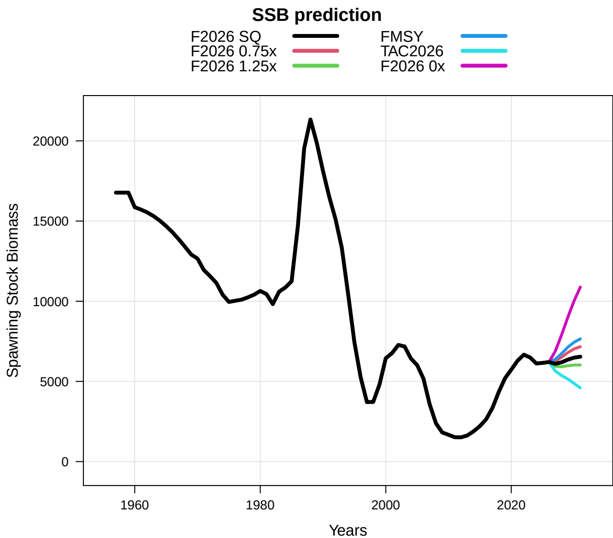
Figure 45: Earlier five-year (2027–2031) spawning biomass projections (thousand tonnes) from h1_1.06.ls under the scenario labels shown in the existing model output.
