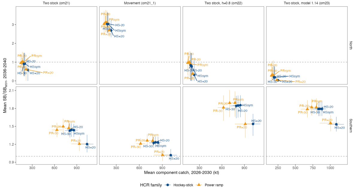
Figure 14: Preliminary component-level trade-offs across the four two-stock robustness OMs.
