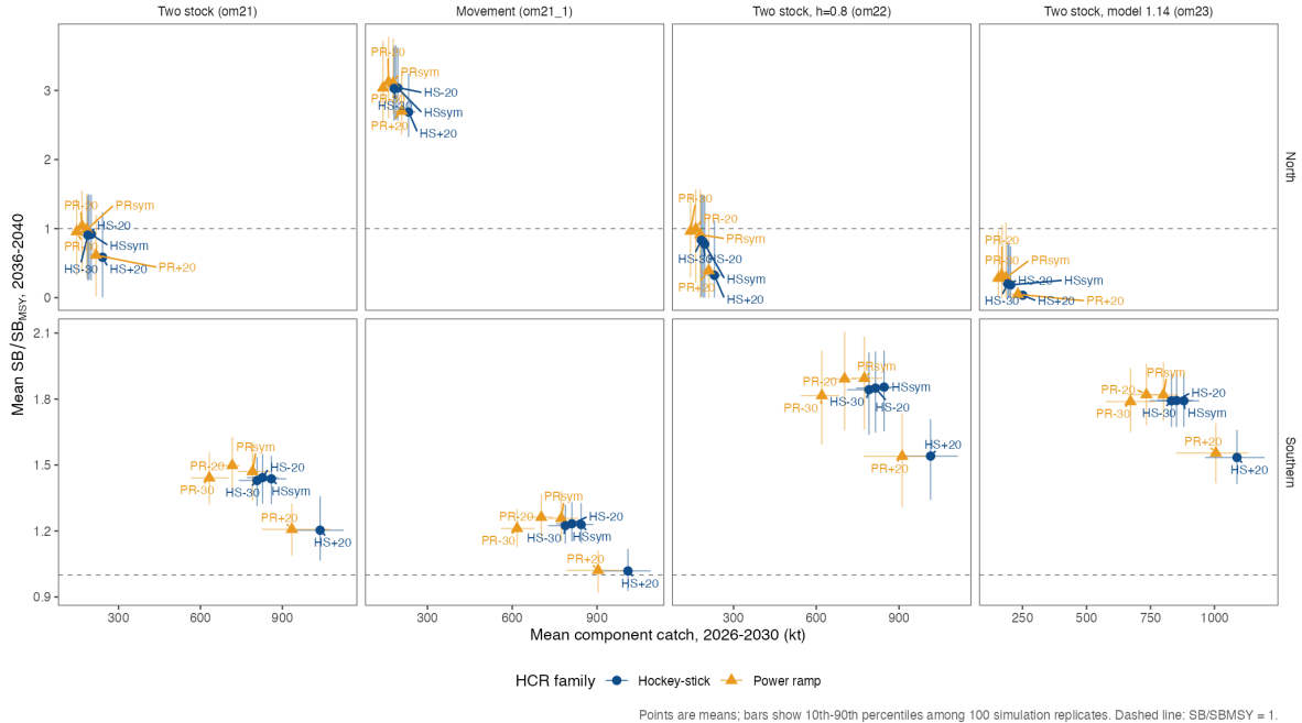
Figure 13: Preliminary component-level trade-offs across the four two-stock robustness OMs.
