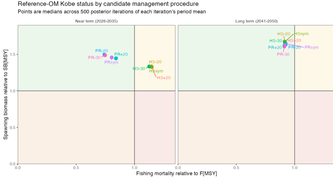
Figure 5: Near- and long-term Kobe plots for the eight CMPs under the reference operating model.
