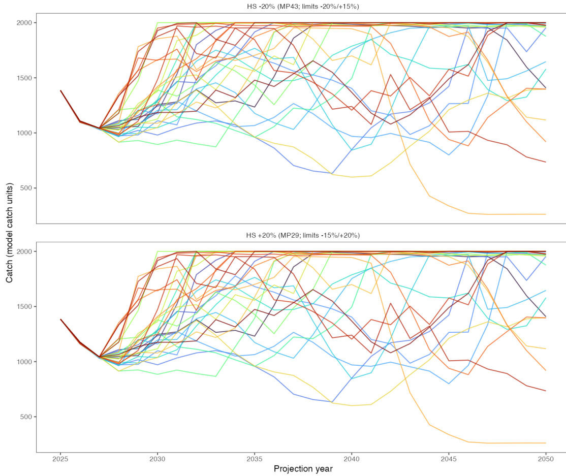
Figure 1: Projected catch trajectories for the same 30 simulation iteration IDs under both hockey-stick MPs in the reference operating model. Each iteration retains the same line color in both panels so matching trajectories can be traced through time and across MPs.
