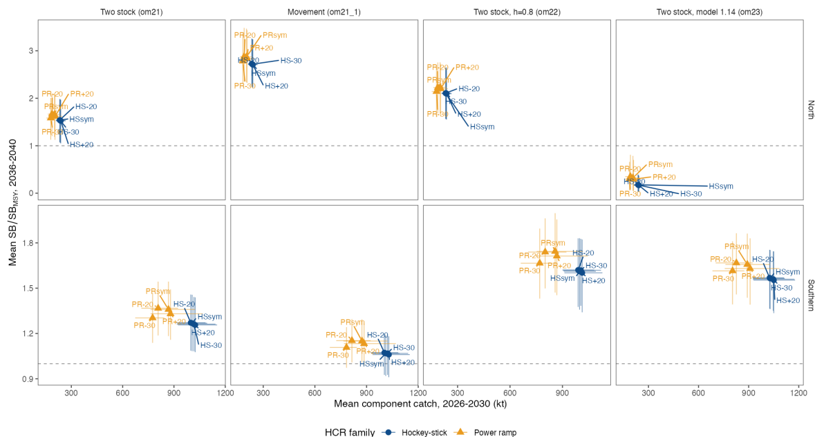
Figure 13: Component-level trade-offs across the four two-stock robustness OMs.
