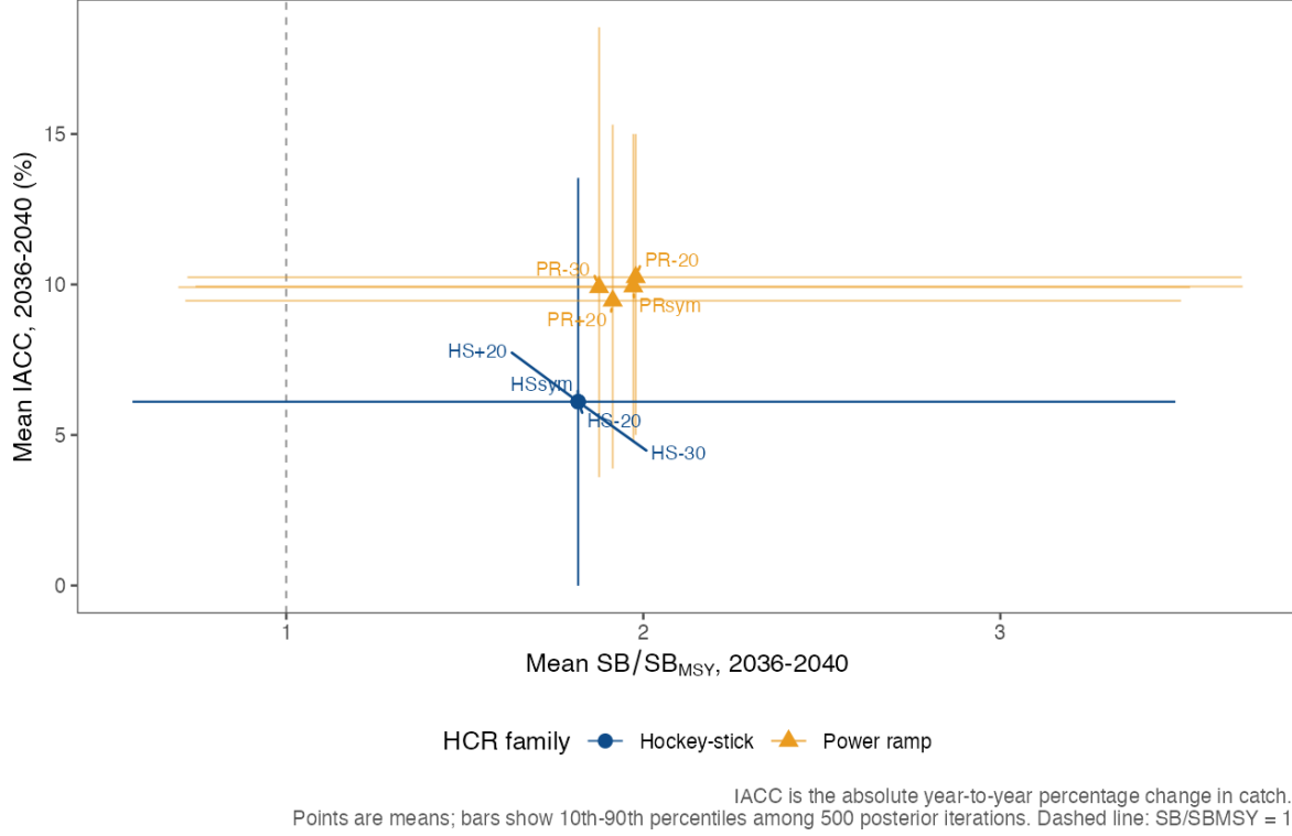
Figure 9: Reference-OM spawning-biomass and interannual-catch-variability trade-off for the eight HS and PR configurations.
