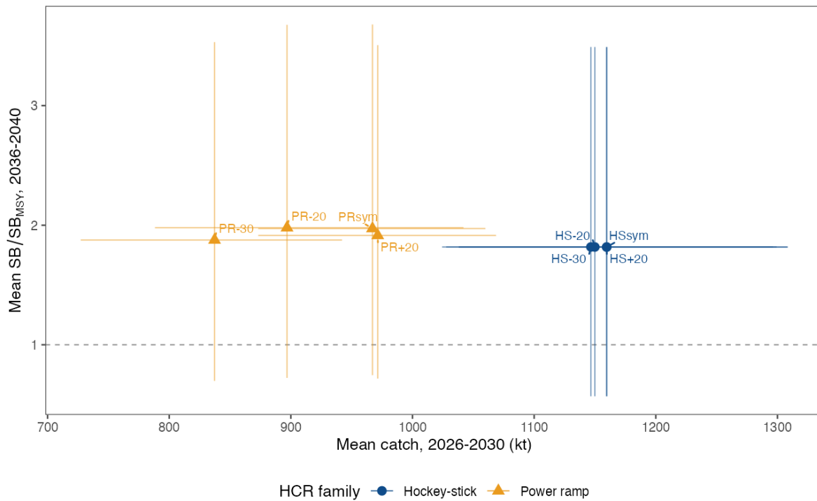
Figure 8: Reference-OM trade-off for the eight HS and PR configurations.
