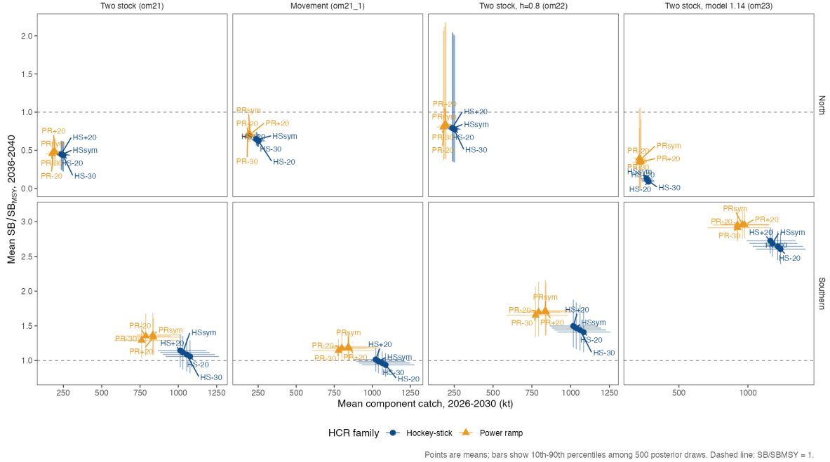
Figure 16: Component-level trade-offs across the four two-stock robustness OMs.
