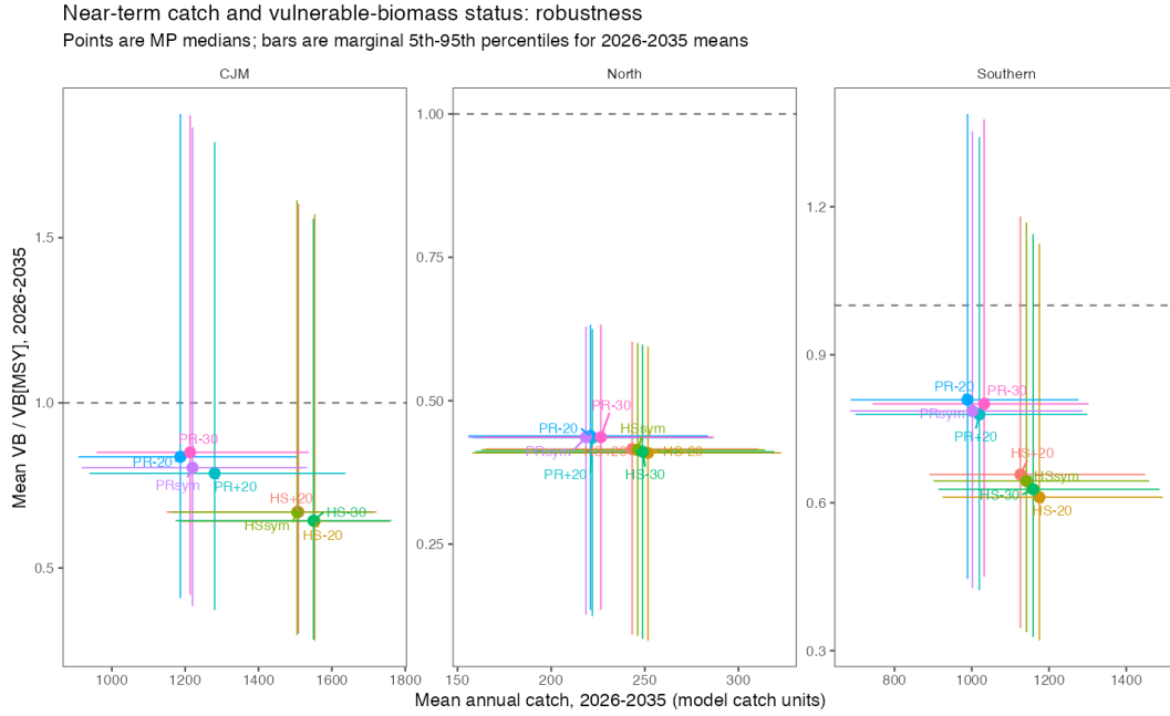
Figure 13: Near-term catch versus VB/VB_{MSY} across robustness operating models, 2026–2035.
