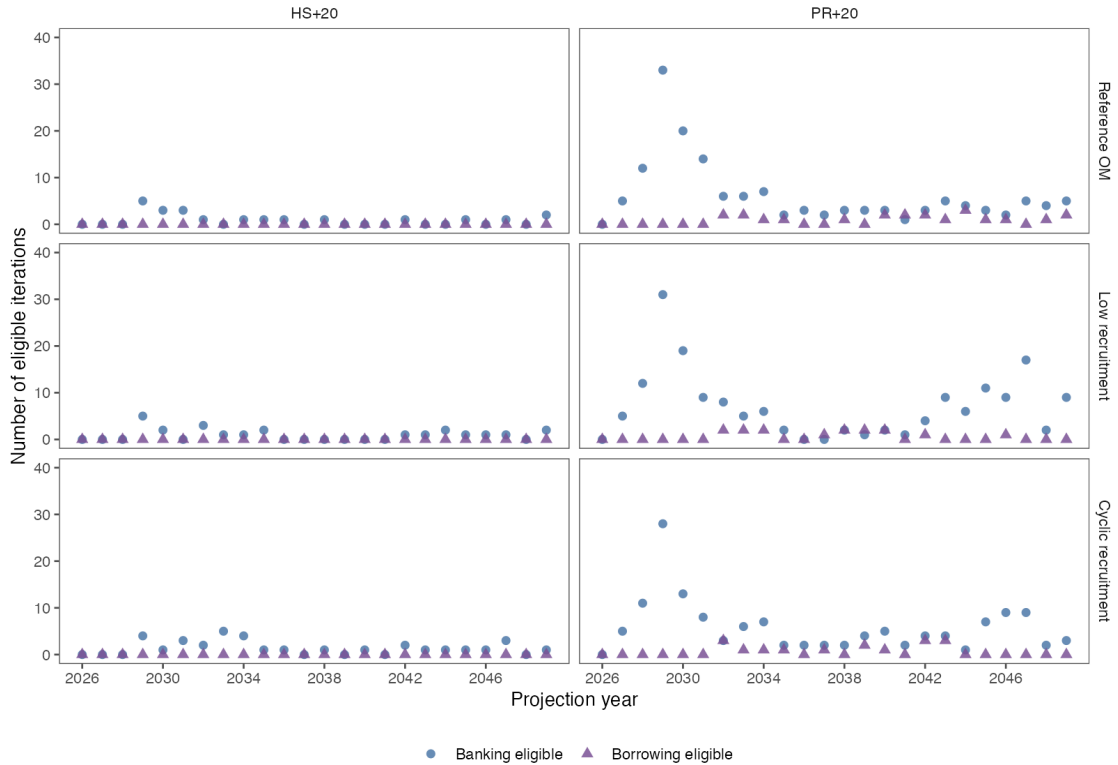
Figure 18: Reconstructed annual eligibility for banking and borrowing in the preliminary 100-iteration runs. Circles denote iterations eligible for banking and triangles denote iterations eligible for borrowing.
