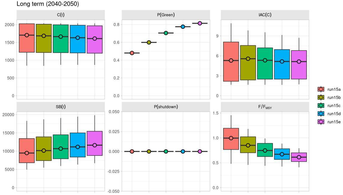
Figure 2: Long-term performance summaries for a set of CMP tuning runs against the reference base model. Panels show catch, P(Green), inter-annual catch variability, spawning biomass, shutdown probability, and F relative to F_{MSY} for runs 15a-15e.
