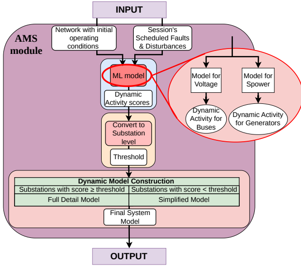
Fig. 2: AMS methodology diagram with parallel Voltage/ S_{\text{power}} models and substation-level conversion
